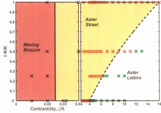
Figure 4.6: Zero temperature phase diagram for K = 10, D = 5 .
