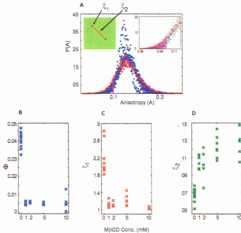
Figure 2.14: Smaller scale changes on cholesterol depletion. (A) The anisotropy distribution is narrow compared to control cells, when cholesterol (using 10mM M \beta CD) is depleted.(B) Accordingly, the fraction of pixels below A=0.1 decreases progressively on increasing M \beta CD concentration. (C and D) The average size of the regions decreases and the distance between them increases.
