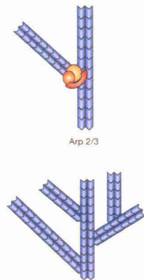
Figure 1.6: ARP Activity (Courtesy [16]): the ARP complex (in orange) binds to an existing actin filament (in blue), enabling cross linking of filaments, and initiating polymerization.
