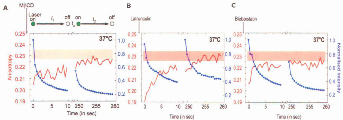
Figure 2.15: Effect of perturbations on Dynamics. The recovery of clusters at 37^{\circ}\text{C} is completely halted when (A)cholesterol, (B)actin or (C)myosin is perturbed.
