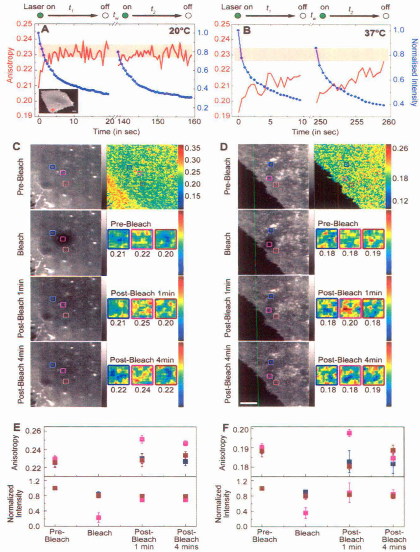
Figure 2.6: Bleaching a small confocal spot on the membrane. A and B are typical traces of anisotropy and intensity during the two bleaching periods 0 \leq t \leq t_1 and t_1 + t_w \leq t \leq t_2 for the temperatures 20^\circ\text{C} and 37^\circ\text{C} . While in A, recovery of anisotropy is almost absent post bleaching, in B, we see a considerable amount of anisotropy recovery. In C and D, three regions are monitored at 20^\circ\text{C} and 37^\circ\text{C} . The central region (in pink) is bleached. The anisotropy in surrounding regions (blue and brown boxes) is almost the same as the central region, and does not increase in time (E and F - 20^\circ\text{C} and 37^\circ\text{C} respectively) during the bleaching of the central region at both temperatures, indicating that these regions do not replenish the central region's nanoclusters via diffusion. At 20^\circ\text{C} , the anisotropy in the pink box does not recover even after 4 minutes post bleaching.
