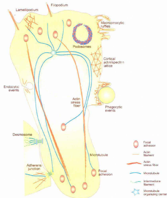
Figure 1.10: Diverse array of actin architectures in the cell. (Courtesy [17])
