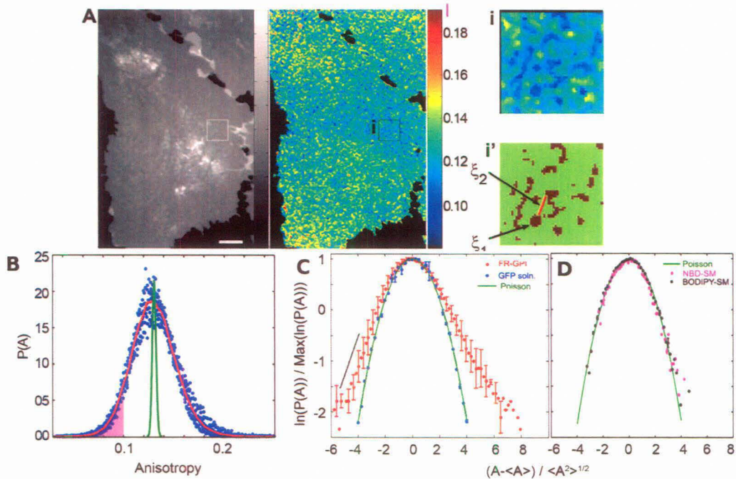
Figure 2.5: Typical features of a cell. (A) The depolarized pixels, with anisotropy values less than a threshold = 0.1 (the pink shaded region in 2.5 B) form ‘islets’ of characteristic size \xi_1 and separation \xi_2 (A i’). (B) A typical distribution can be ascribed to the control cells (red curve), which is considerably broader than a Poisson distribution of clusters and monomers (green curve). (C) The typical distribution has exponential tails as opposed to the Poisson distribution and a solution of GFP molecules. (D) Bulk membrane markers, such as short chained lipids (Sphingomyelin labeled with fluorescent dyes NBD and BODIPY), in contrast, do not have exponential tails and coincide with the Poisson distribution.
