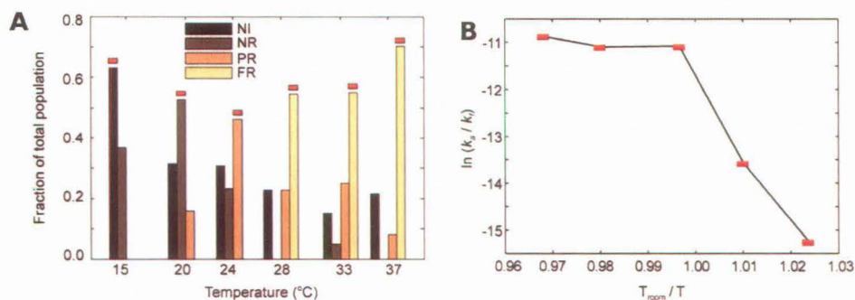
Figure 2.10: Arrhenius Plot. (A) Histogram representing the relative abundance of the class FR for 37°C, 33°C and 28°C, PR for 24°C, NR for 20°C and NI for 15°C. (B) An Arrhenius Plot using the most probable values of the rates at these temperatures shows a switching behaviour at 24°C.
