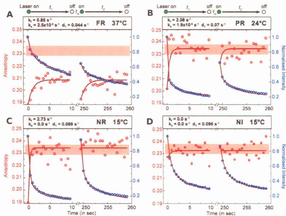
Figure 2.9: Representative fits for each of the classes. The panels A, B, C and D contain intensity and anisotropy traces and fit parameters ( k_a , k_f and d_1 ) for each of the classes FR, PR, NR and NI respectively.
