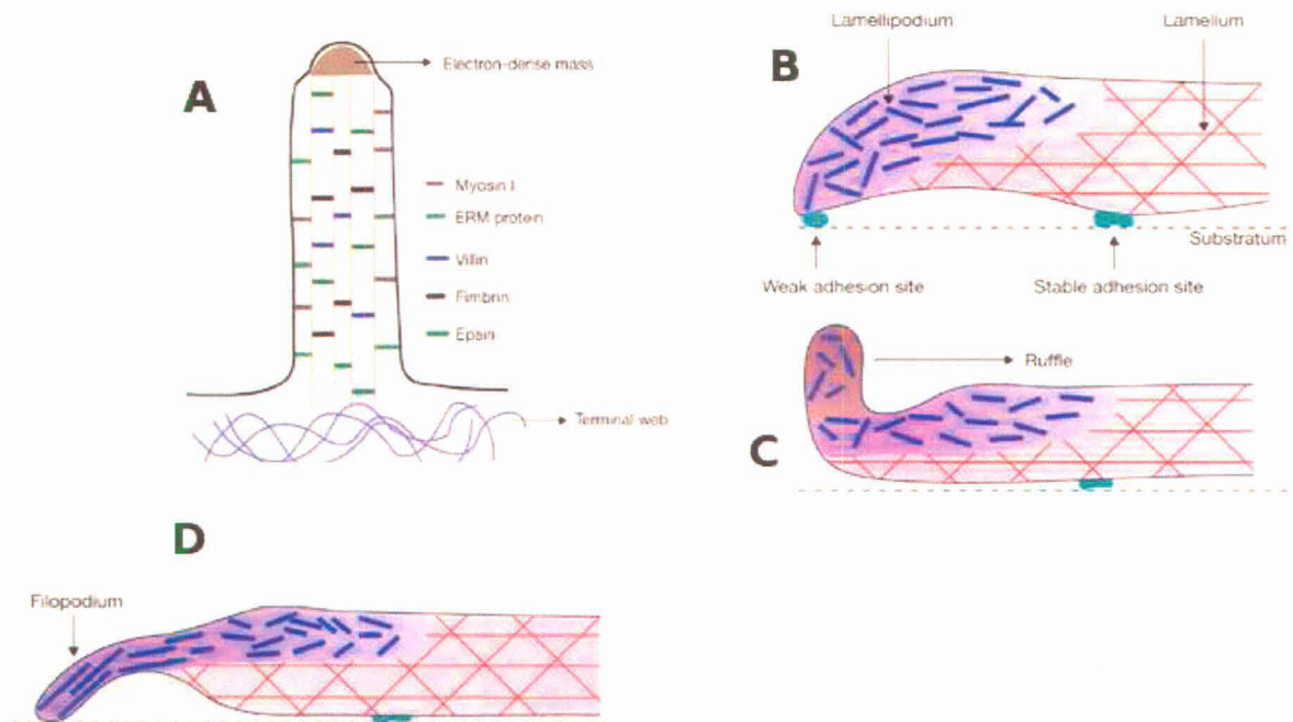
Figure 1.9: Various Architectures of Actin (Courtesy [16]): A. Microvilli containing vertical bundles of crosslinked actin. (B, C, D) Lamellipodia, ruffles and filipodia, containing polymerizing filaments that aid in locomotion.
