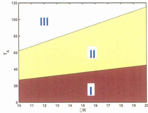
Figure 4.17: \zeta - T_A phase diagram
