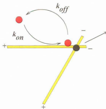
Figure 4.20: Passive Particle dynamics. A Passive Particle (in red) hops on and off a cross-linked pair of filaments and is advected along by the filaments
