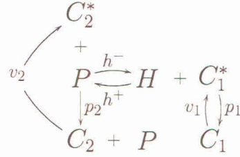
Figure 3.6: A Simplified Network of The Reactions
