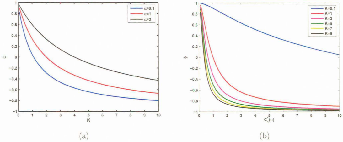
Figure 3.7: The order parameter \phi , switching between high and low levels of CDC42 (a) as a function of ARHGAP10 availability, for various values of \alpha , at v_1/\bar{p}_1 = v_2/\bar{p}_2 = 1 (b) as a function of ARF1 ( C_1^*(\infty) ) for various value of K , at v_2/\bar{p}_2 = 1 , \alpha = 1 .
