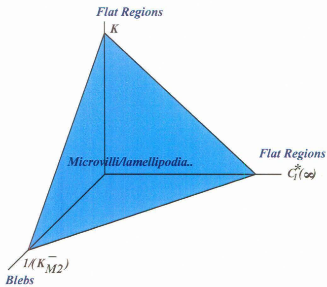
Figure 3.9: Qualitative Phase Diagram of actin architectures
