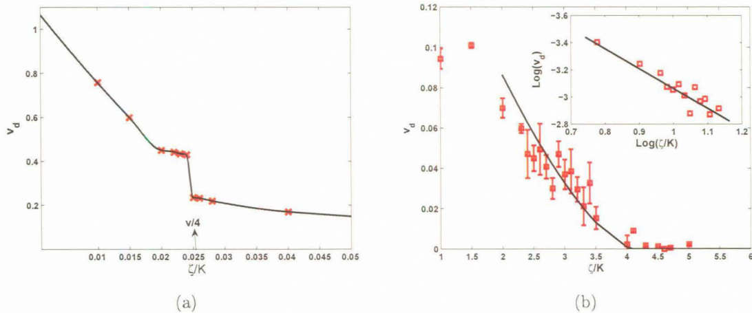
Figure 4.5: Velocity \langle c\mathbf{n} \cdot \hat{e}_x \rangle vs \zeta/K . (a) At the boojum-street transition, the velocity shows a jump (b) At the street-lattice transition, the velocity shows a continuous power law decay to zero satisfying v \sim (\zeta/K - 4)^{1.7}
