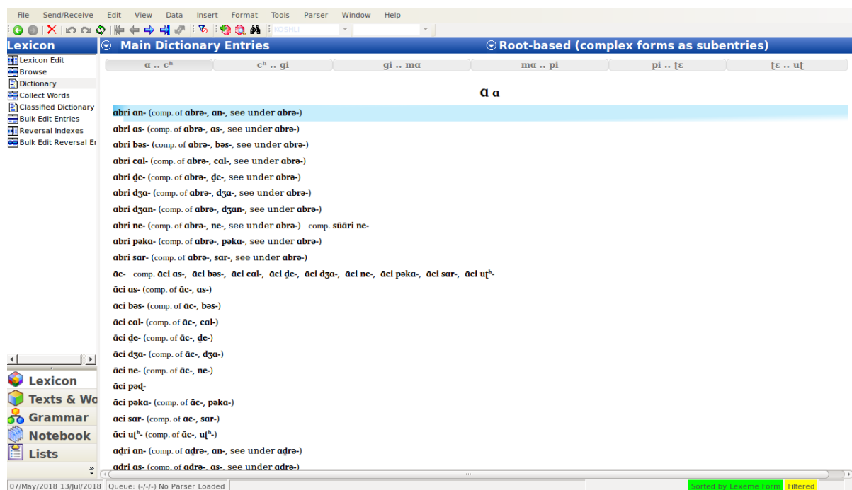
Figure 6 Root-Based View
