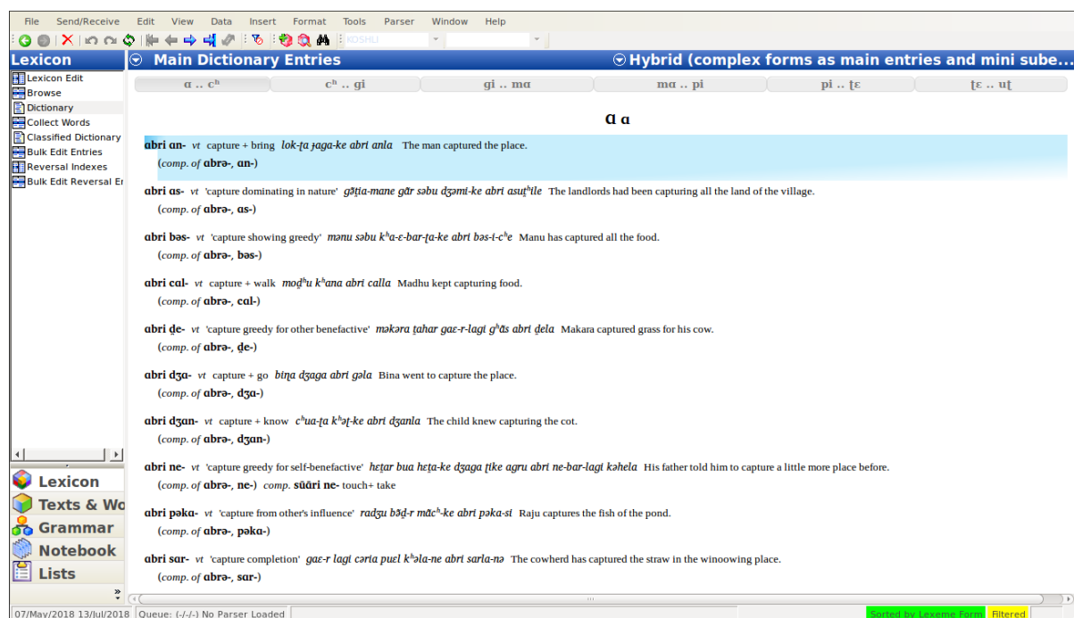
Figure 7 Hybrid view
